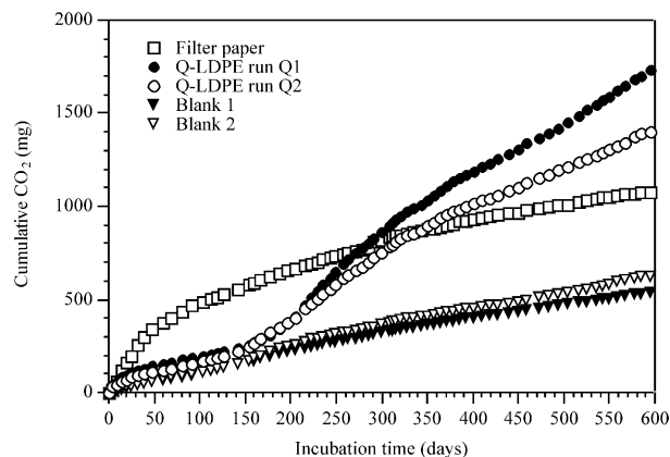
Fig. 2. Cumulative \text{CO}_2 emissions of filter paper, and thermally fragmented Q-LDPE at two different concentrations and blanks in a soil burial respirometric test.
