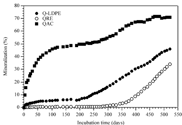
Fig. 7. Mineralization profiles of Q-LDPE, residue to solvent extraction (QRE), and acetone extract (QAC) of Q-LDPE sample in soil burial test.
