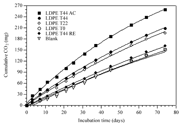
Fig. 13. Cumulative CO 2 emissions of acetone extract of the LDPE specimen submitted to 44 days oxidative thermal treatment (LDPE T44 AC), entire LDPE film specimens collected after 22 (LDPE T22) and 44 (LDPE T44) days thermal treatment, residues to extraction (LDPE T44 RE), original LDPE film (LDPE T0) and blank in a soil burial test.
