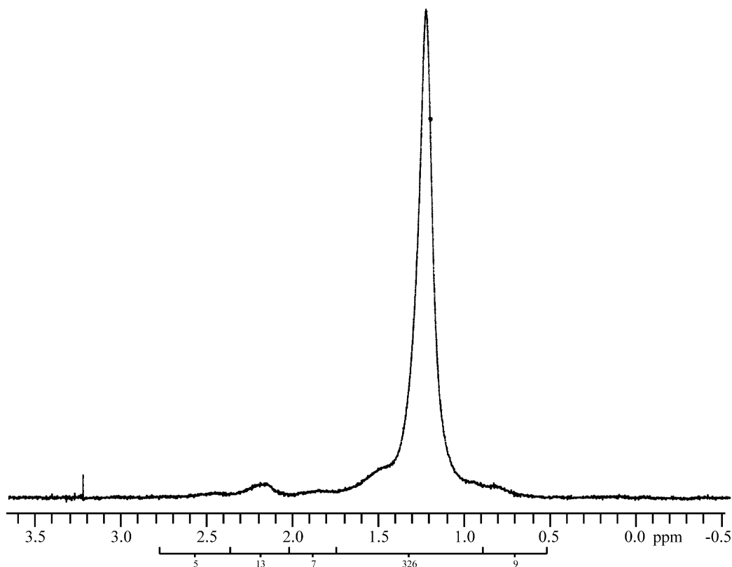
Fig. 9. ^1\text{H} NMR spectra of residue to solvent extraction (QRE sample) of thermally fragmented Q-LDPE sample.
