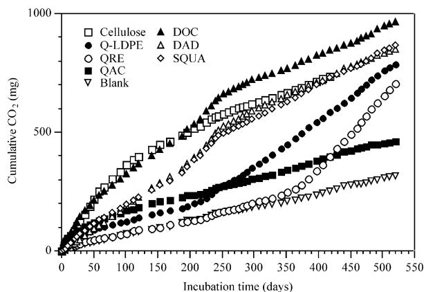
Fig. 6. Cumulative \text{CO}_2 emissions of Q-LDPE, residue to solvent extraction (QRE), acetone extract (QAC) of Q-LDPE sample, and reference aliphatic hydrocarbons (Docosane DOC, \alpha,\omega -docosandioic acid DAD, and squalane SQUA) in soil burial test.
