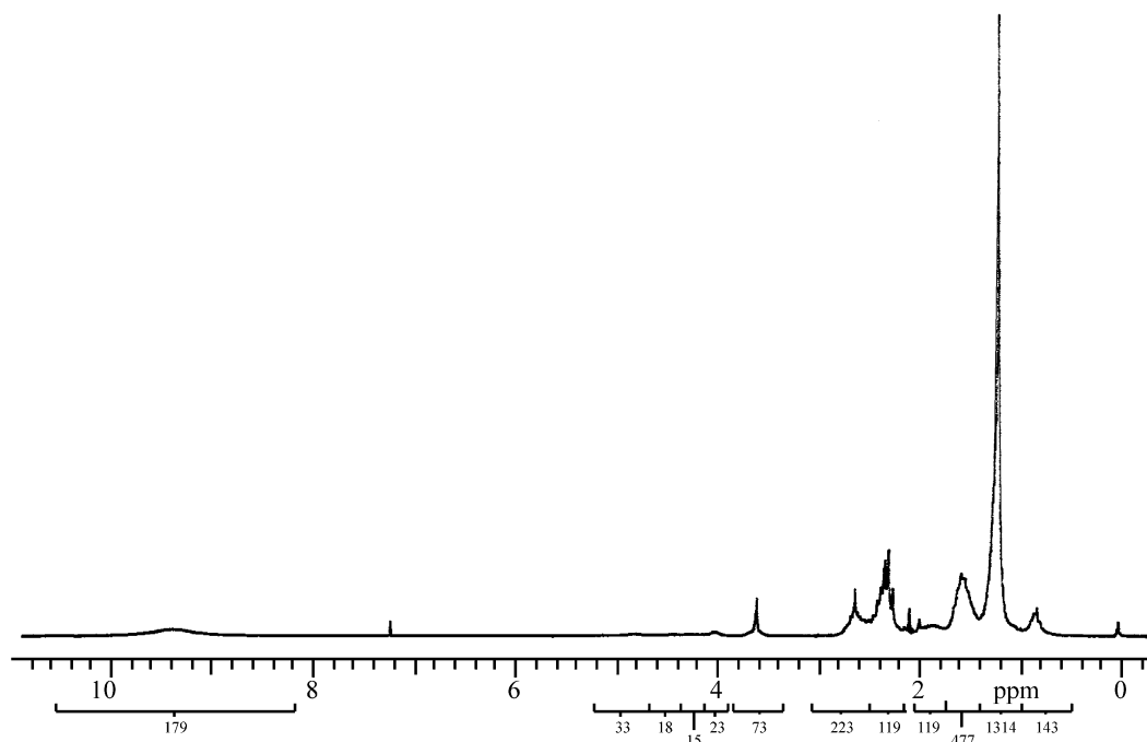
Fig. 8. ^1\text{H} NMR spectra of QAC extracted with acetone from thermally fragmented Q-LDPE sample.
