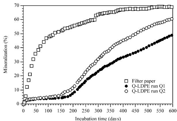
Fig. 3. Mineralisation profiles of thermally fragmented Q-LDPE samples and filter paper in soil burial test.
