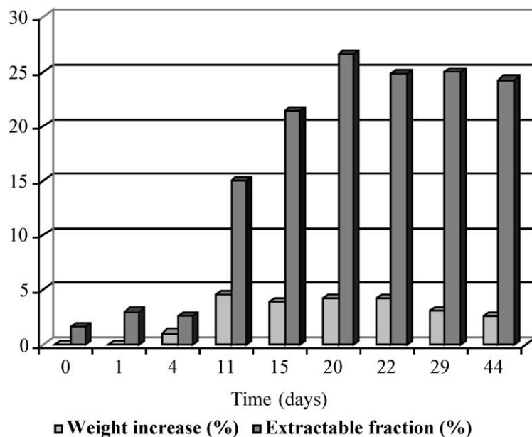
Fig. 11. Increase of dry weight and solvent extractable fraction of LDPE blown film specimens submitted to thermal degradation test.
