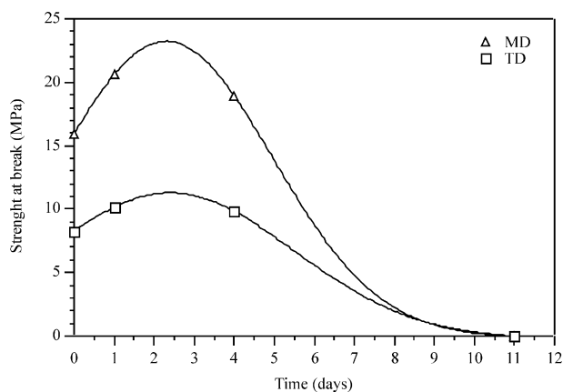
Fig. 12. Strength variation of LDPE specimens retrieved from the thermal treatment.
