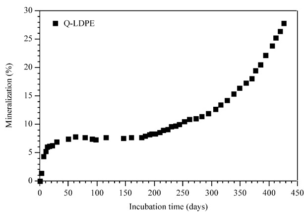
Fig. 10. Mineralization profiles of thermally fragmented Q-LDPE sample in mature compost incubation medium.
