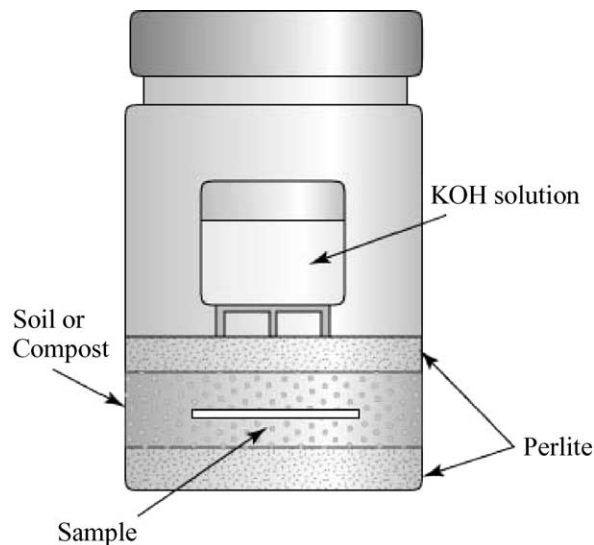
Fig. 1. Biometer flask for simulated soil burial and mature compost biodegradation tests.
